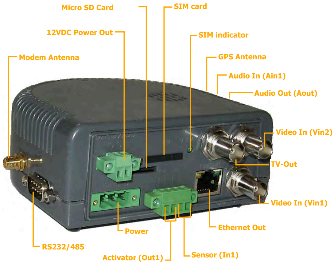
Figure 2: CVG-M connectors
