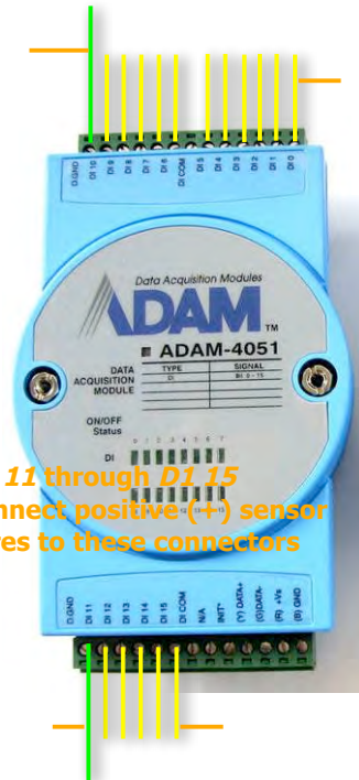
Figure 13: Connecting sensors to the ADAM-4051 module
