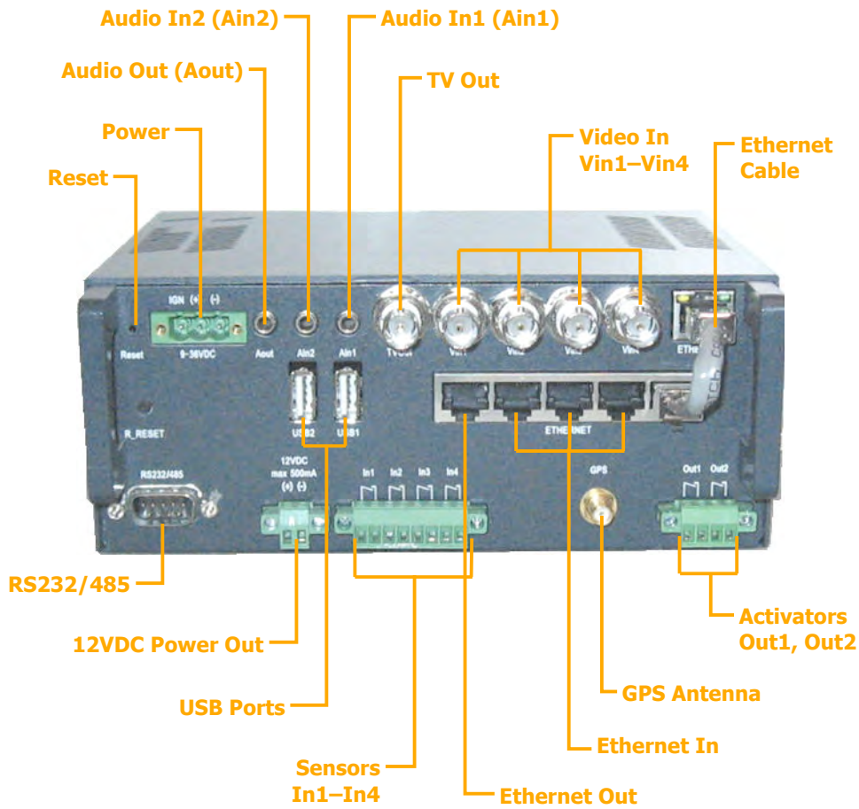
Figure 5: MVG connectors and controls
