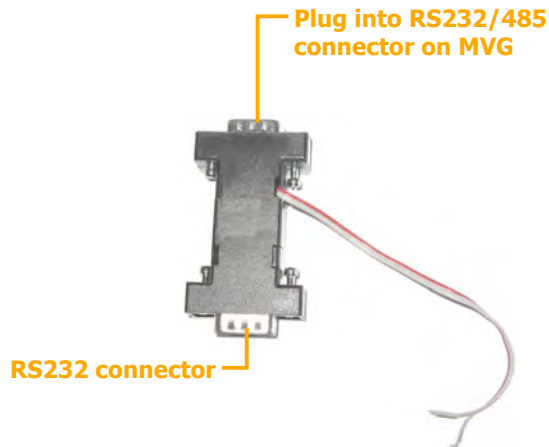
Figure 16: RS232/485 adapter
