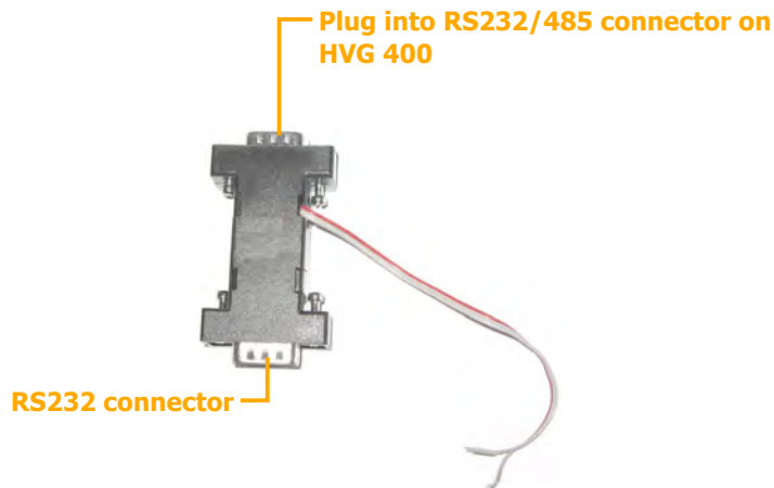
Figure 20: RS232/485 adapter
