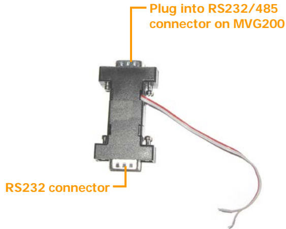
Figure 24: RS232/485 adapter
