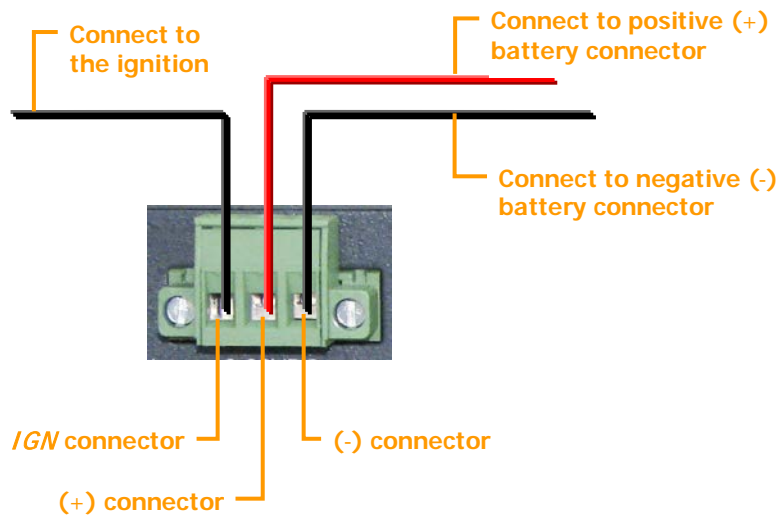
Figure 33: Connecting the MVG200 to the vehicle battery and the ignition
