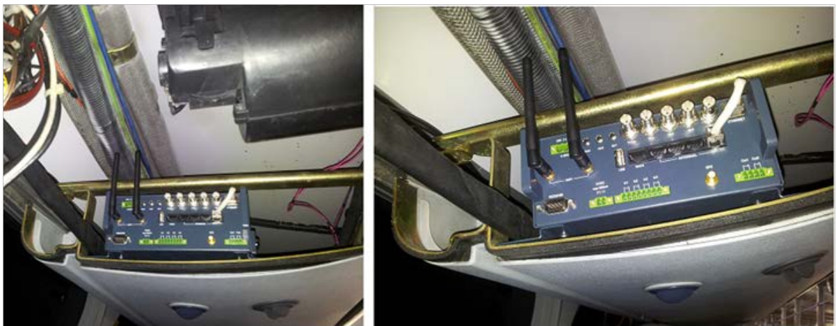
Figure 3: Video Gateway installed in the air-conditioning duct of a bus
