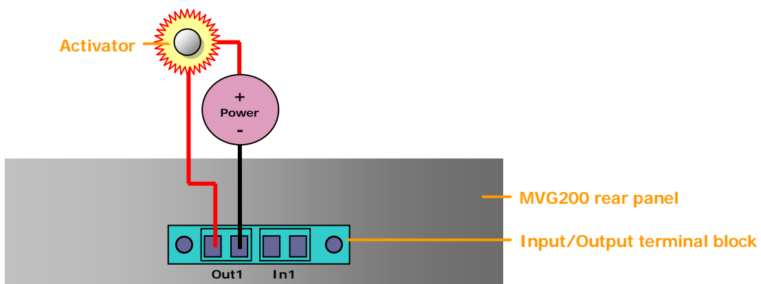
Figure 20: Connecting an activator that has its own power supply
