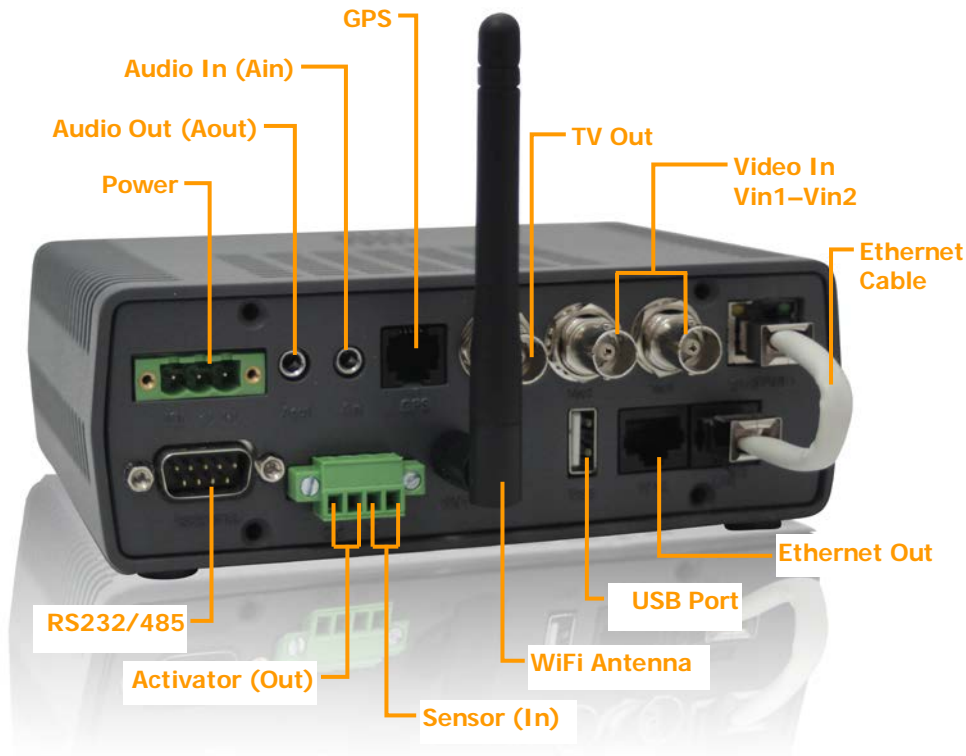
Figure 7: MVG200 connectors and accessories
