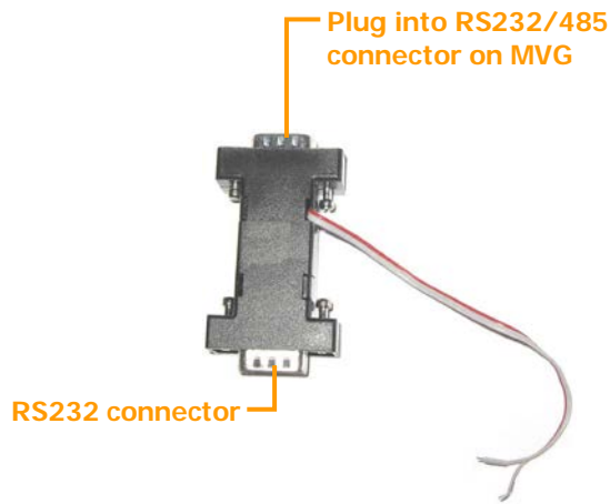
Figure 18: RS232/485 adapter
