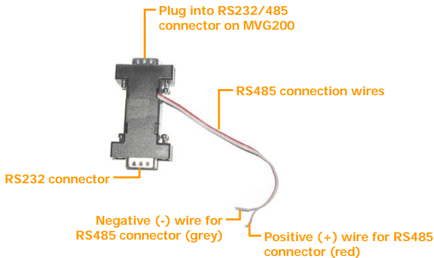
Figure 12: RS232/485 adapter
