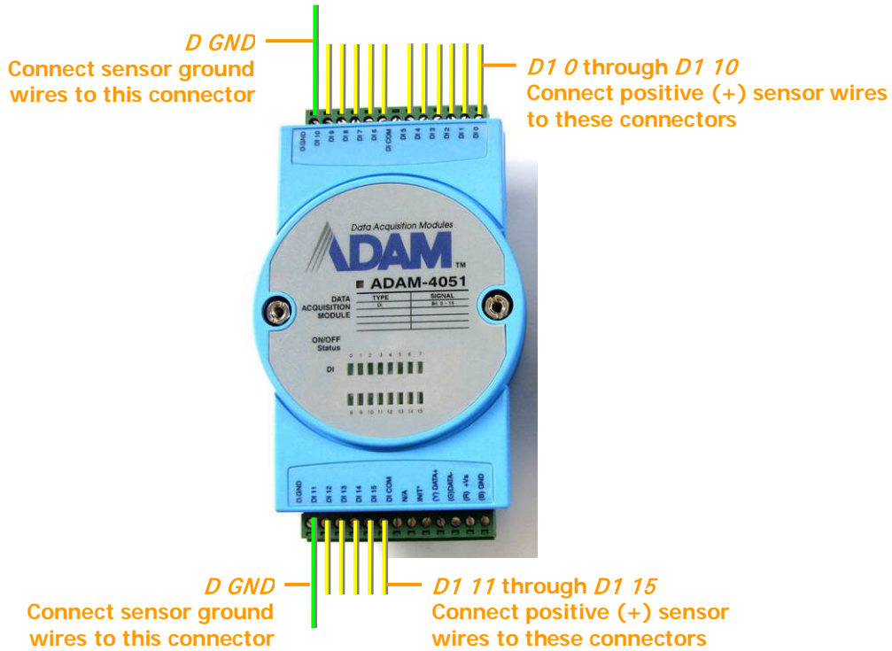
Figure 17: Connecting sensors to the ADAM-4051 module
