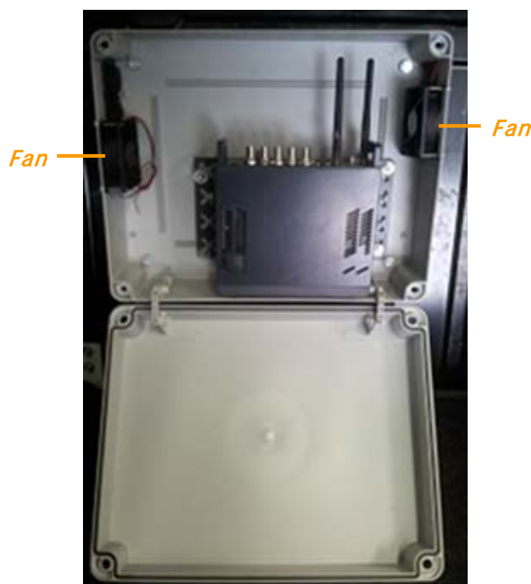
Figure 1: Video Gateway installed in an insulated plastic container with two fans
