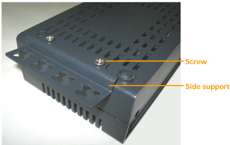
Figure 6: Support attached to the bottom of the MVG200
