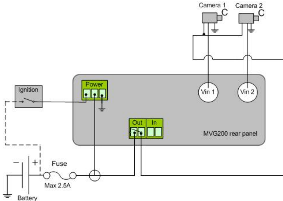
Figure 8: Connecting cameras to the power supply through an Activator connector
