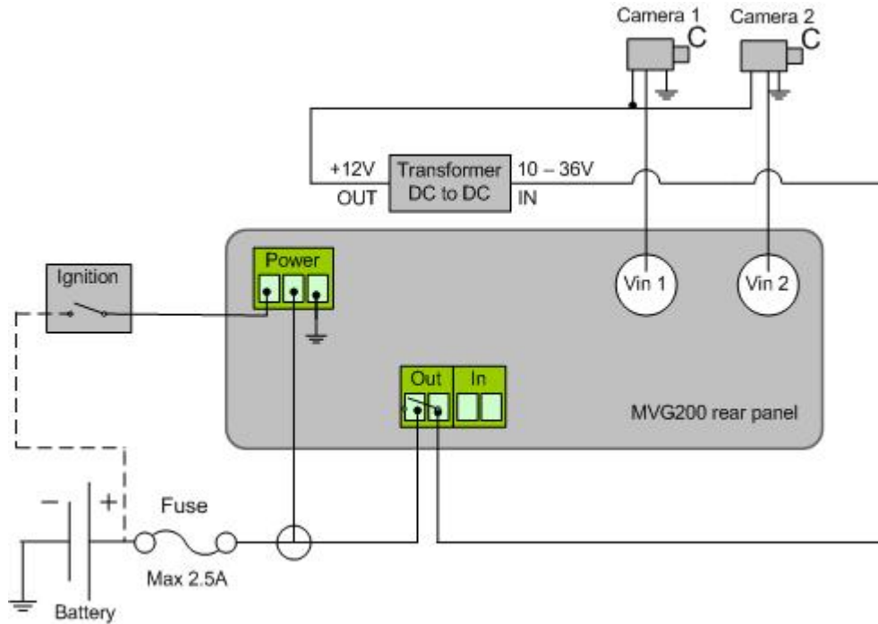
Figure 9: Placing a transformer between the vehicle battery and the devices drawing power from it
