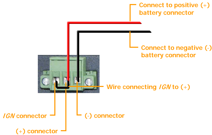
Figure 34: Connecting the IGN connector to the (+) connector when a connection to the ignition is not required
