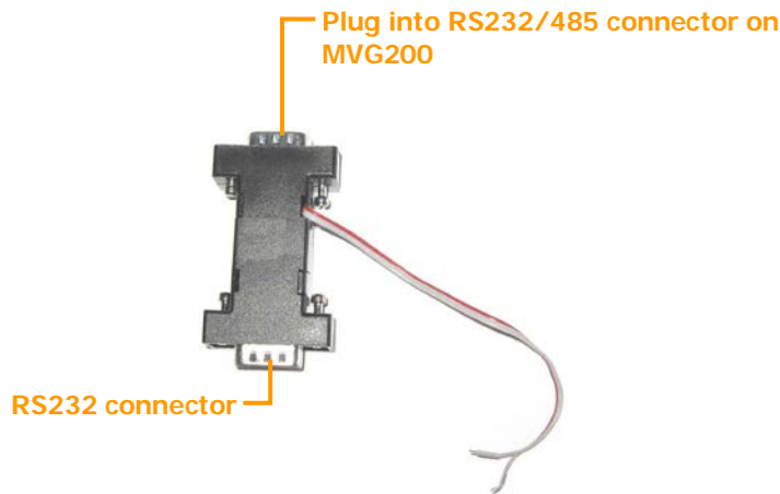
Figure 22: RS232/485 adapter
