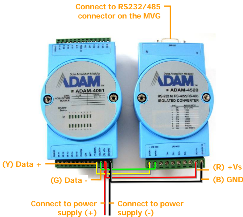
Figure 19: Connecting the module to the converter, the MVG200, and the power supply
